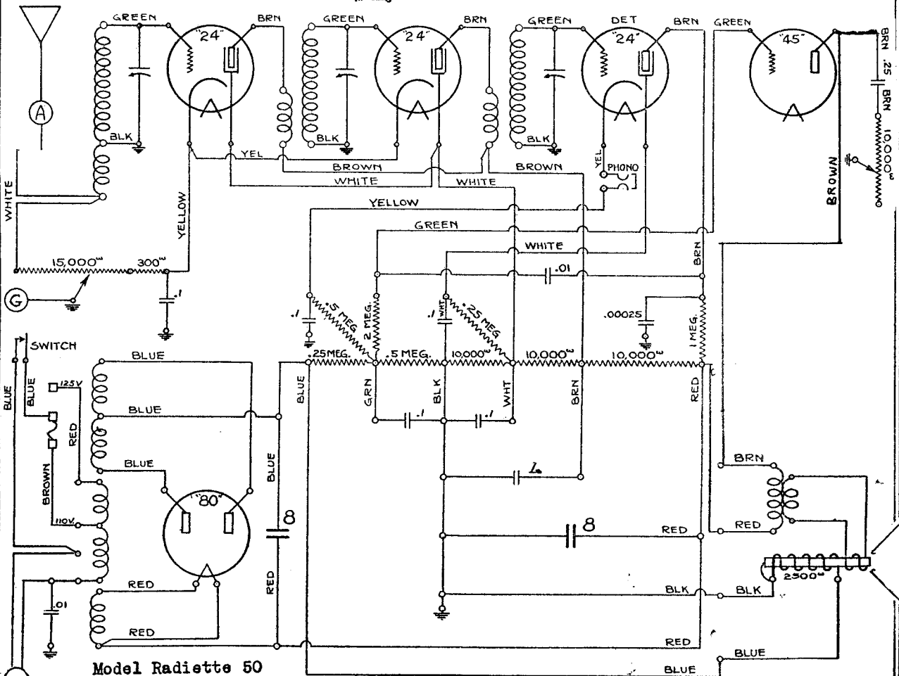
Model Radiette 50
